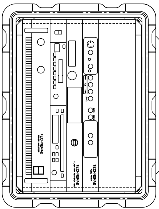
FRONT VIEW (WITH LIDS REMOVED)
